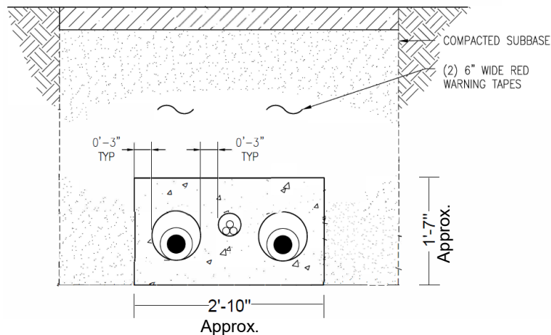
HVDC Duct Bank Cross Section
