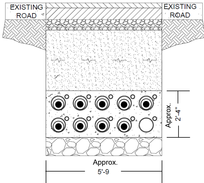
HVAC Duct Bank Cross Section
