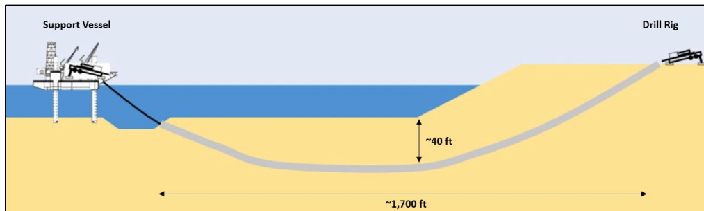
Horizontal Directional Drilling (image courtesy of DEME Offshore US)
